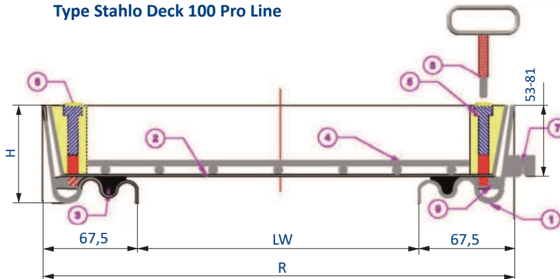
Type Stahlo Deck 100 Pro Line
